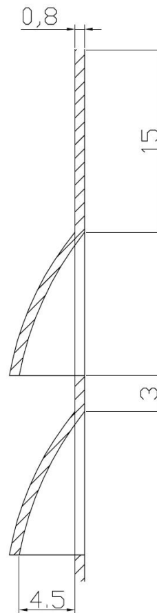
CROSS SECTION THROUGH VENT
