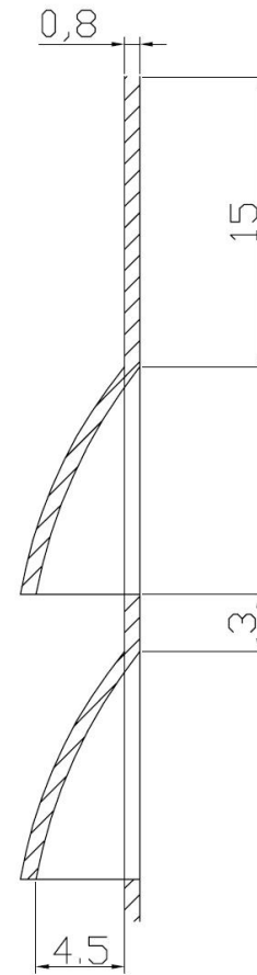
CROSS SECTION THROUGH VENT
