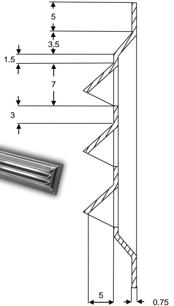
CROSS SECTION THROUGH VENT
