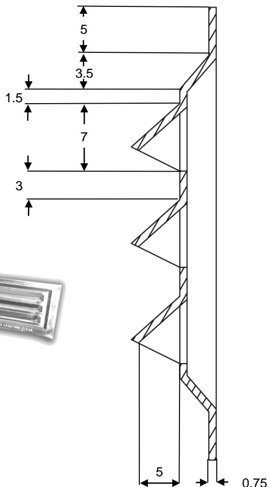
CROSS SECTION THROUGH VENT
